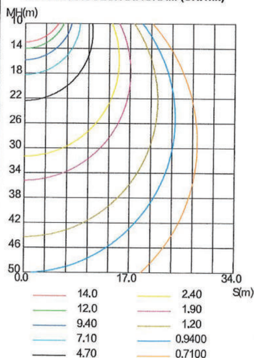
C0 PLANE ISOLUX DIAGRAM (UNIT:lx)
